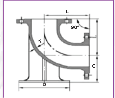
90° Flanged Duckfoot Bend
